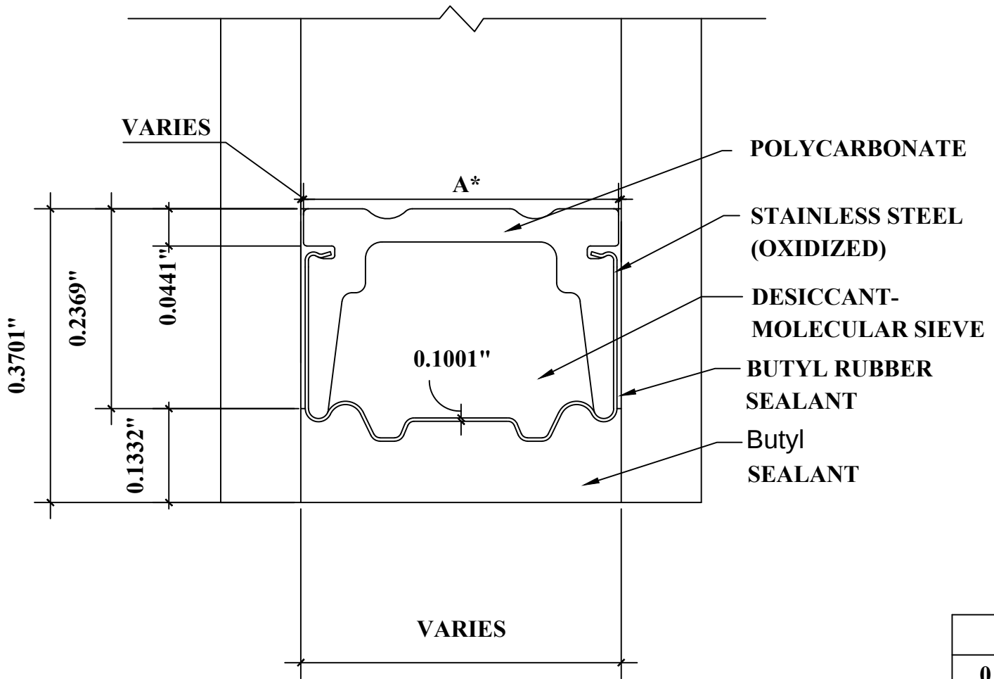
DETAIL FOR THERMAL MODELING OF ROLLTECH CHROMATECH ULTRA SPACER (TS-D)
